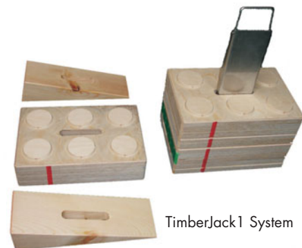
TimberJack - Laminated Stabilisation Blocks
